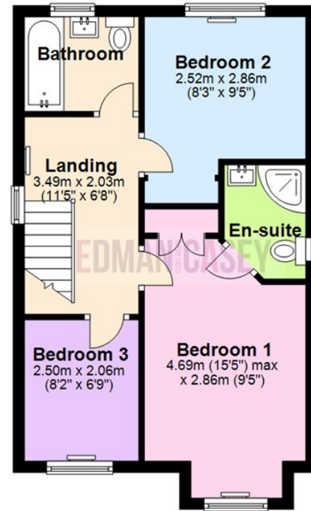
First Floor Approx. 40.3 sq. metres (434.0 sq. feet)
